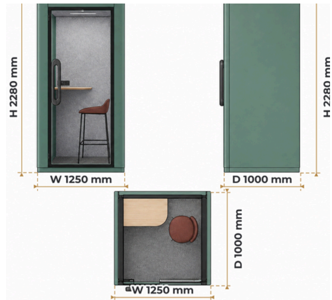
MOVUSH M1 Work — Core · H2280 · all dimensions in mm
