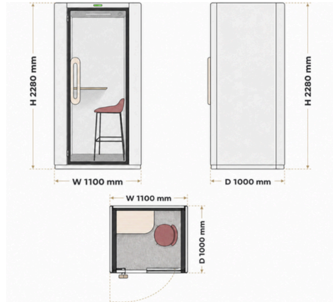
MOVUSH M1 Call — Core · H2280 · all dimensions in mm
