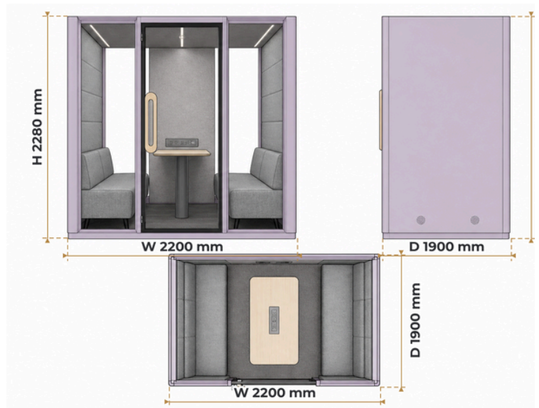
MOVUSH M6 — Core · H2280 · all dimensions in mm
