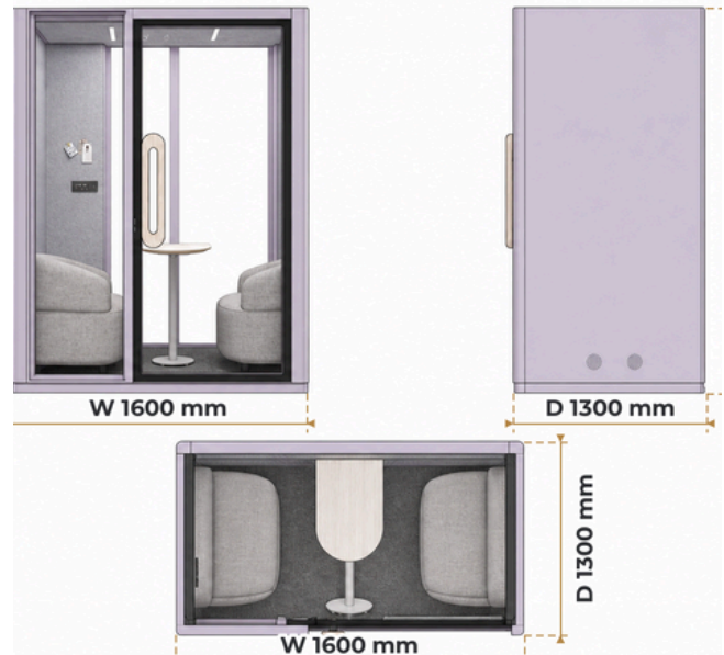
MOVUSH M2 — Core · H2280 · all dimensions in mm
